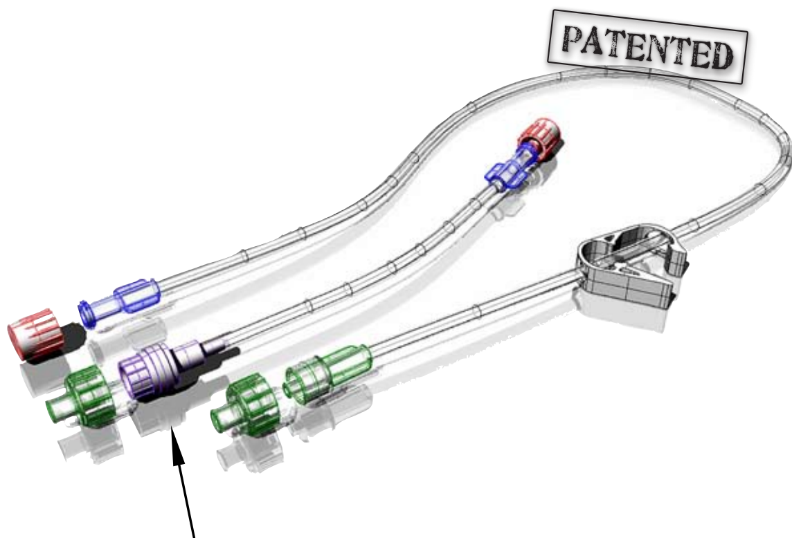
Non-Return Valve with disconnect feature
